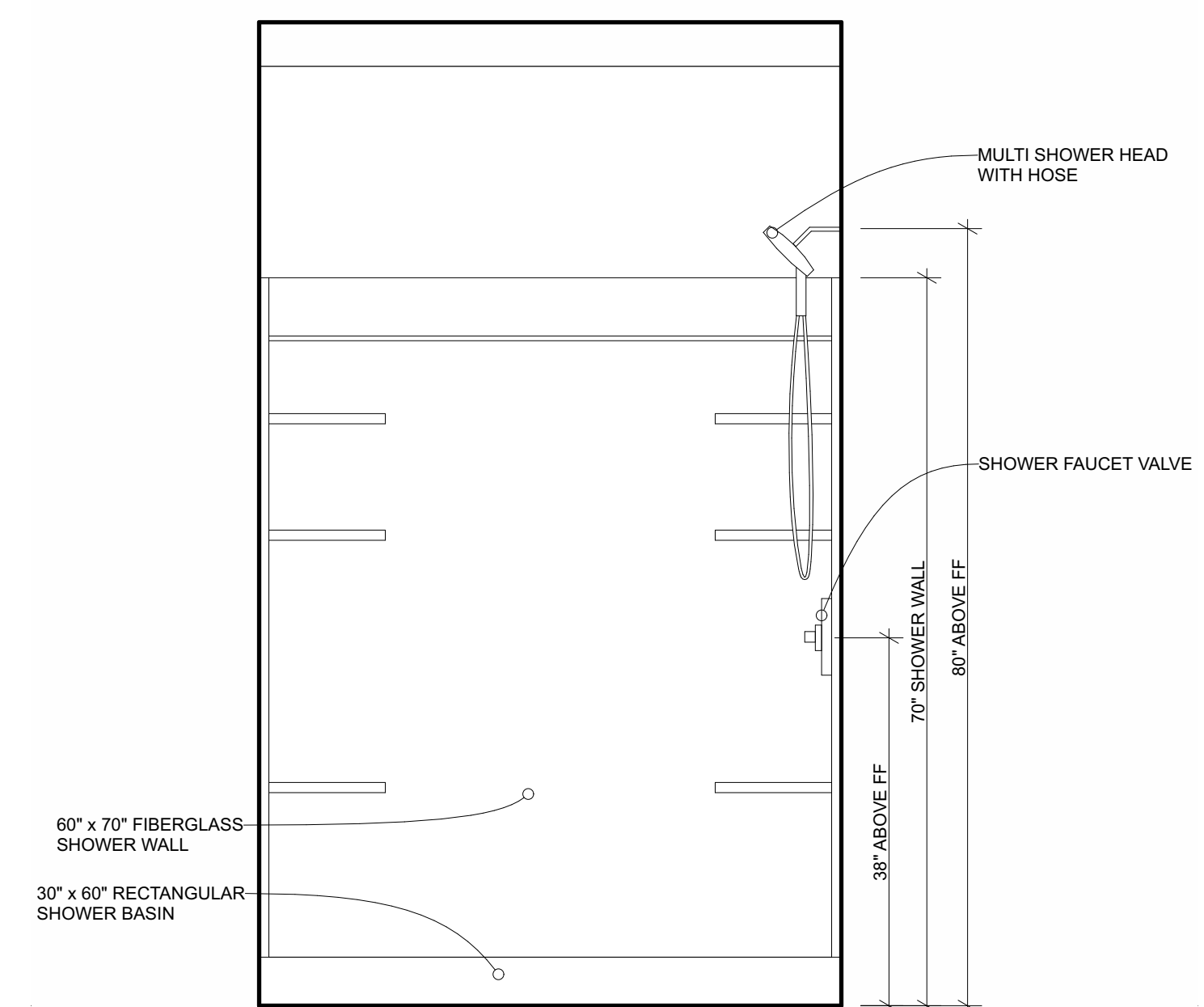
4 SINGLE UNIT SHOWER WALL SCALE: 3/4" = 1'-0"
