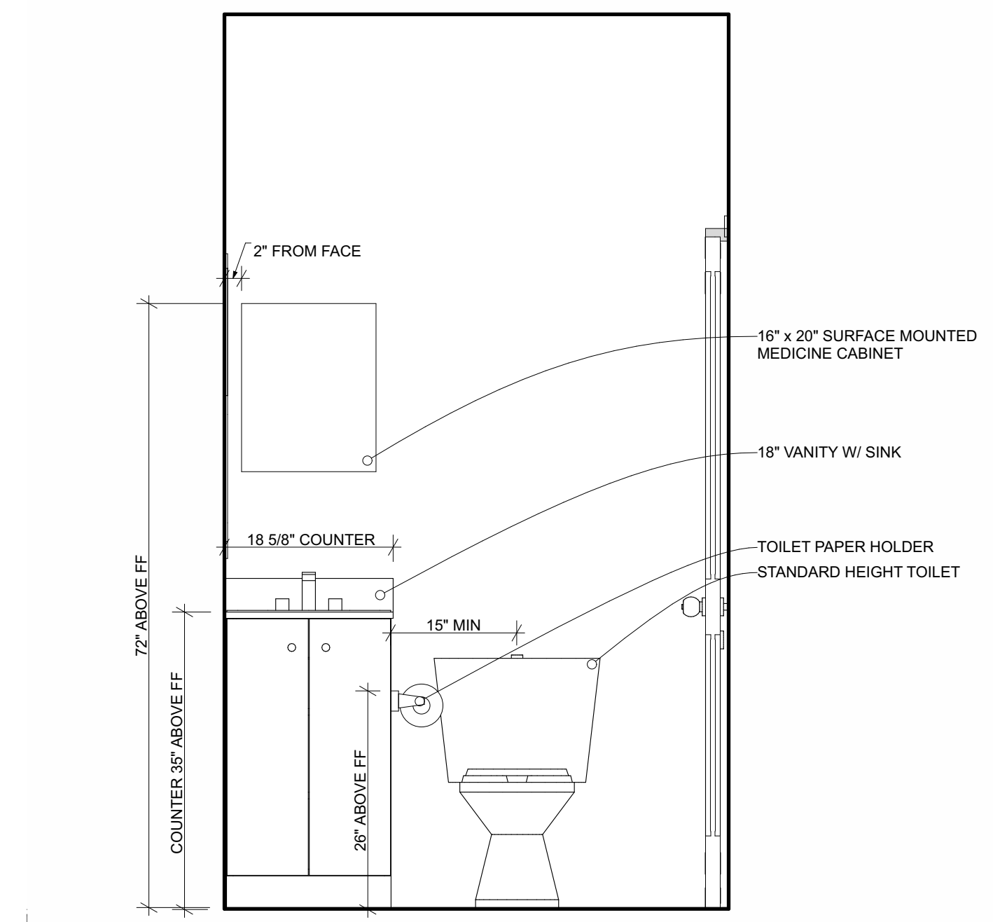
1 SINGLE UNIT SINK WALL SCALE: 3/4" = 1'-0"
