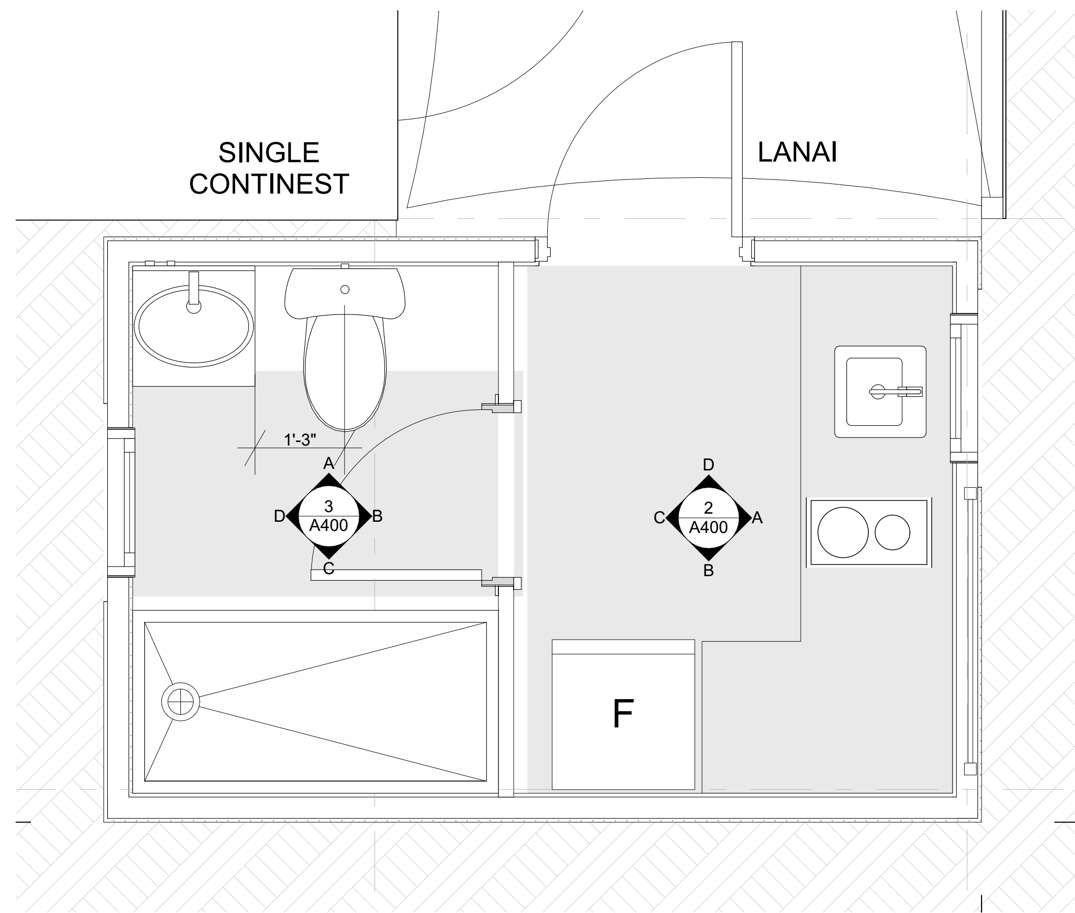
5 ENLARGED SINGLE UNIT SHED SCALE: 3/4" = 1'-0"
