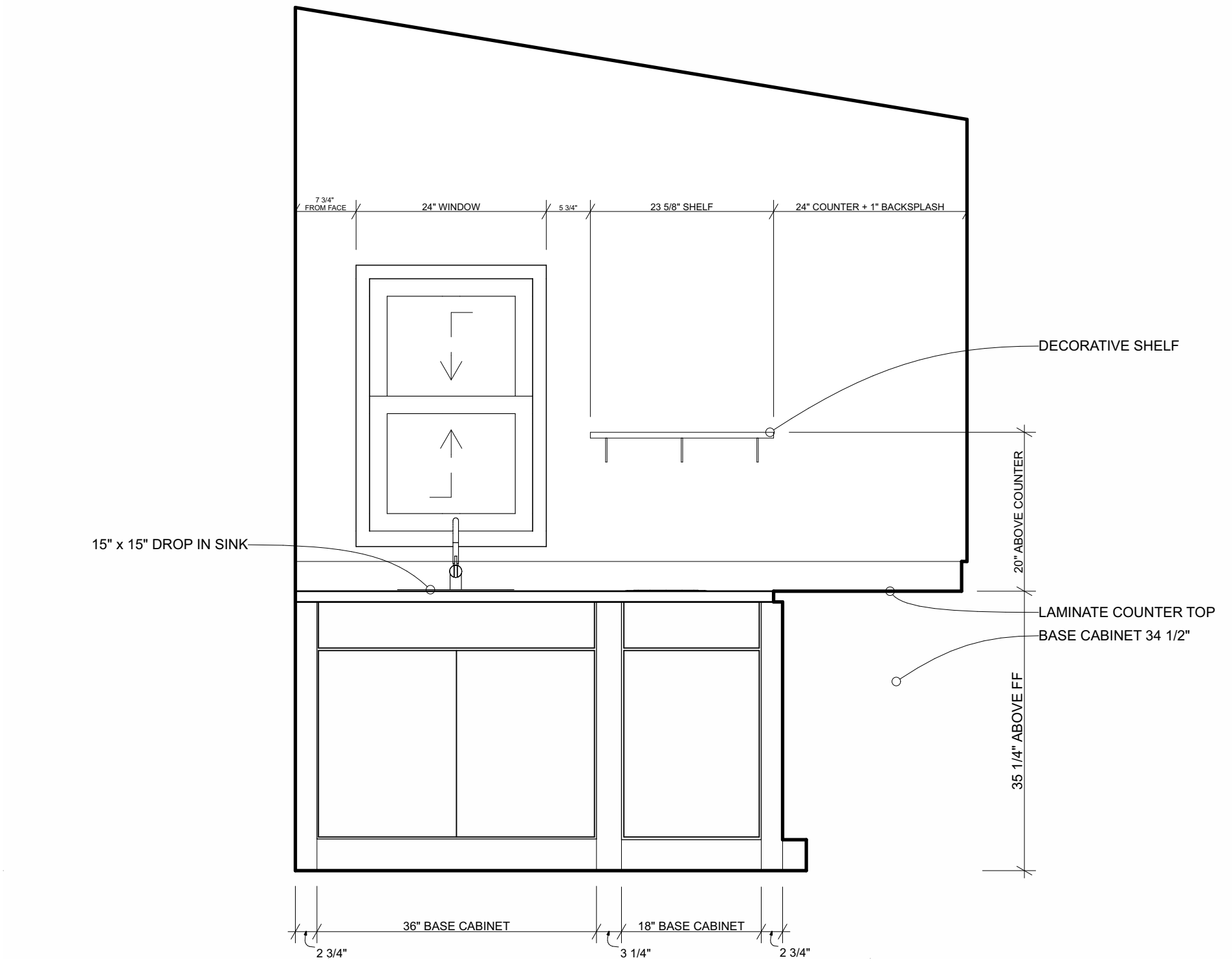
3 A202 KITCHEN WINDOW WALL SCALE: 3/4" = 1'-0"
