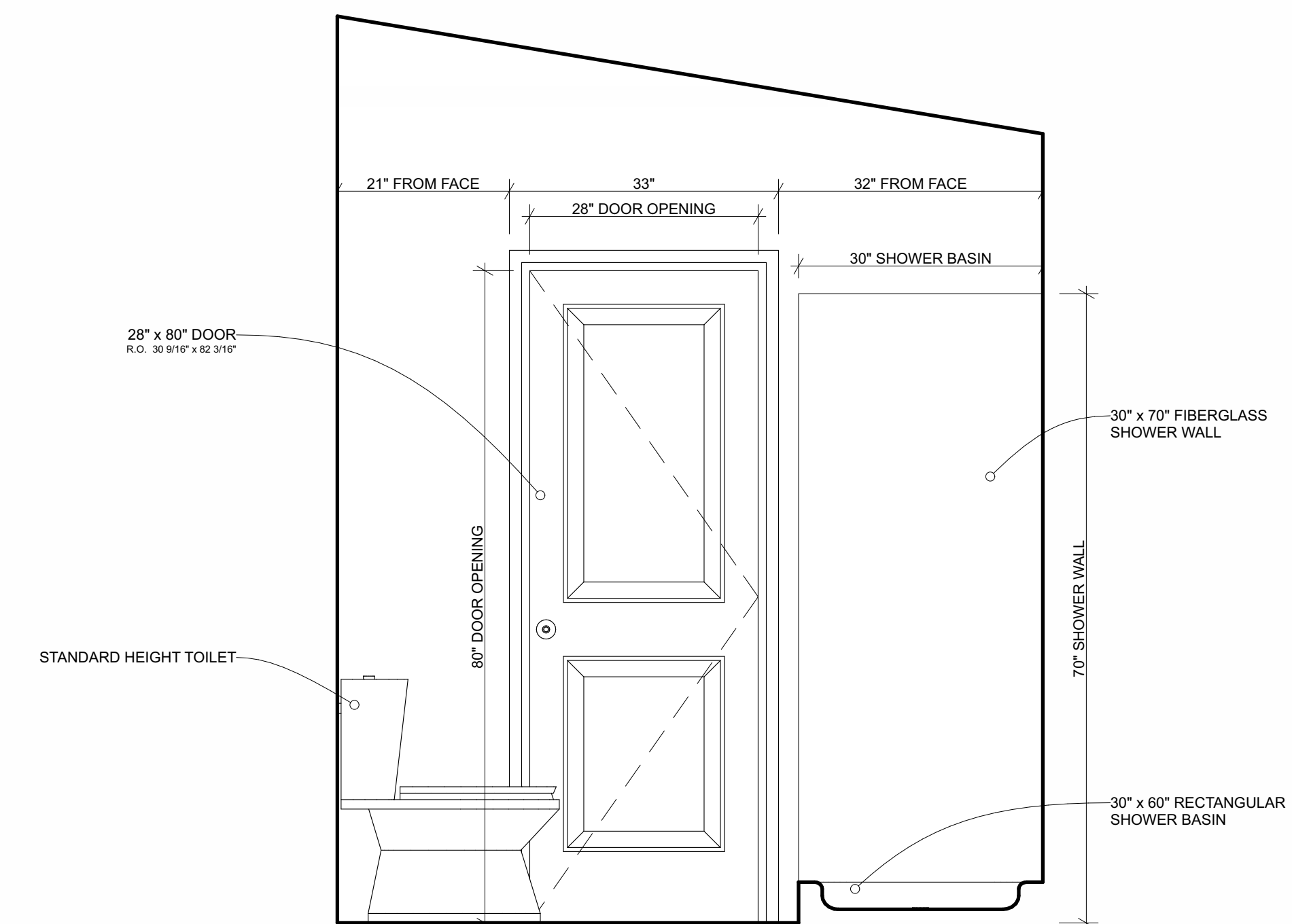
3 SINGLE UNIT ENTRANCE WALL SCALE: 3/4" = 1'-0"
