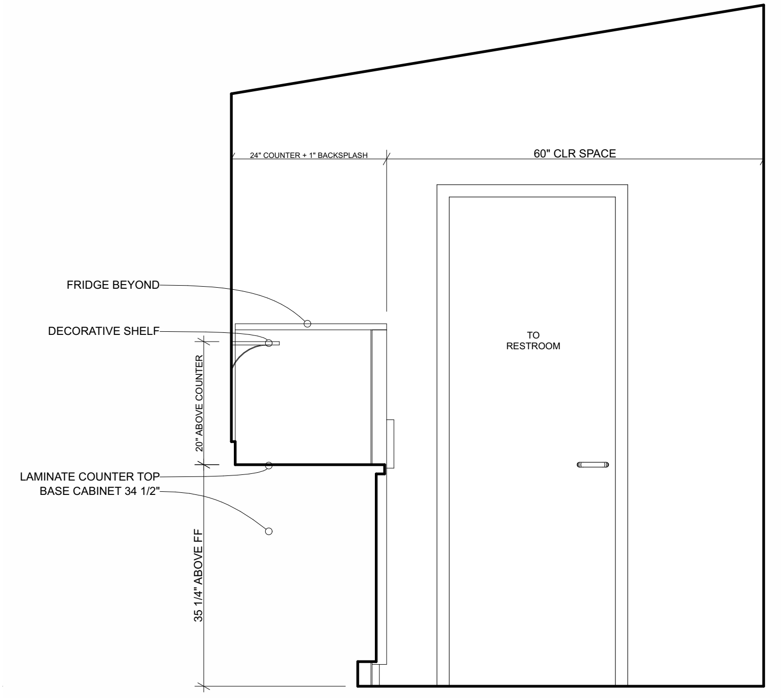
2 A202 RESTROOM DOOR WALL SCALE: 3/4" = 1'-0"
